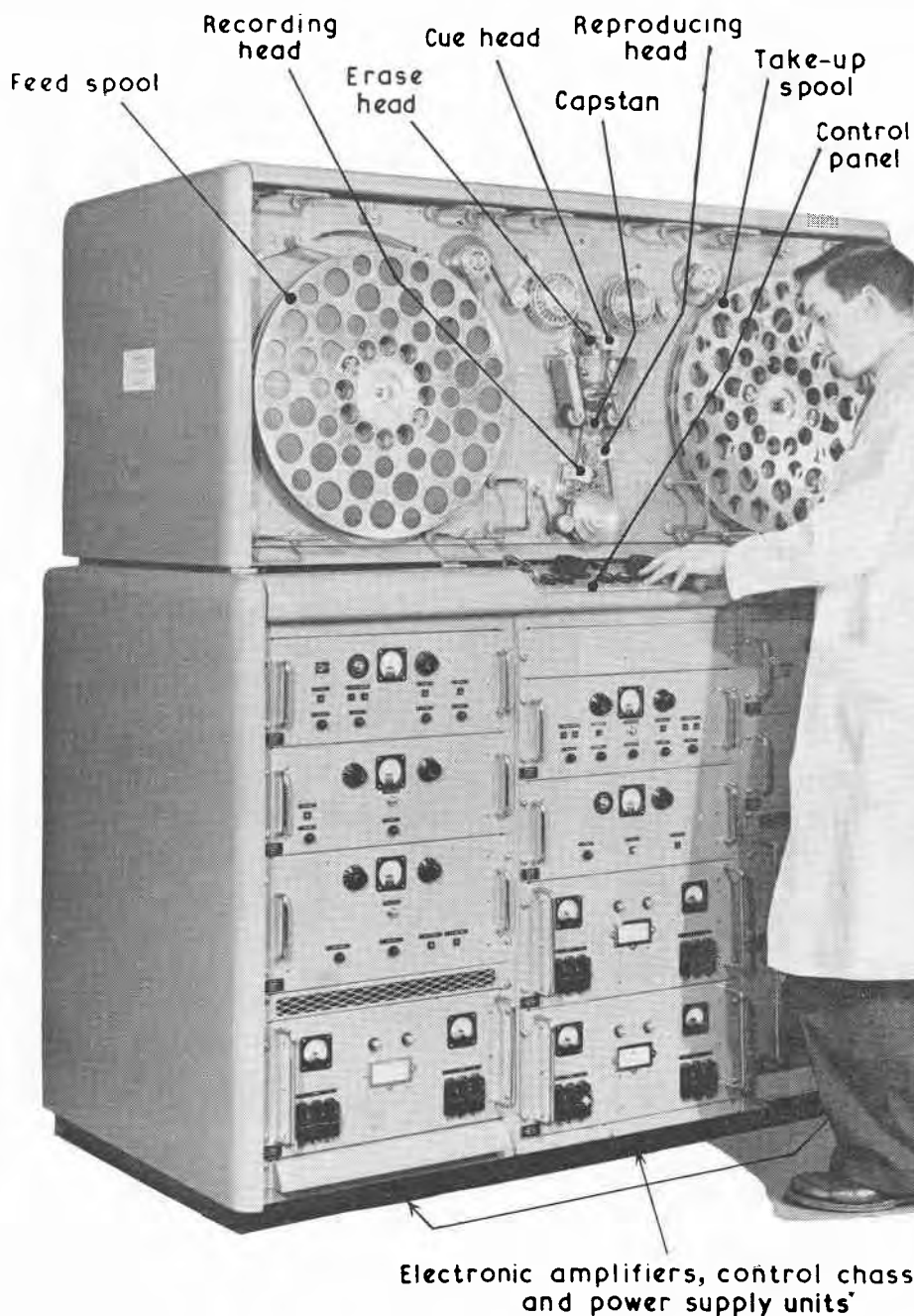
VERA (Vision Electronic Recording Apparatus) designed and built by BBC engineers for recording television programmes on magnetic tape.
